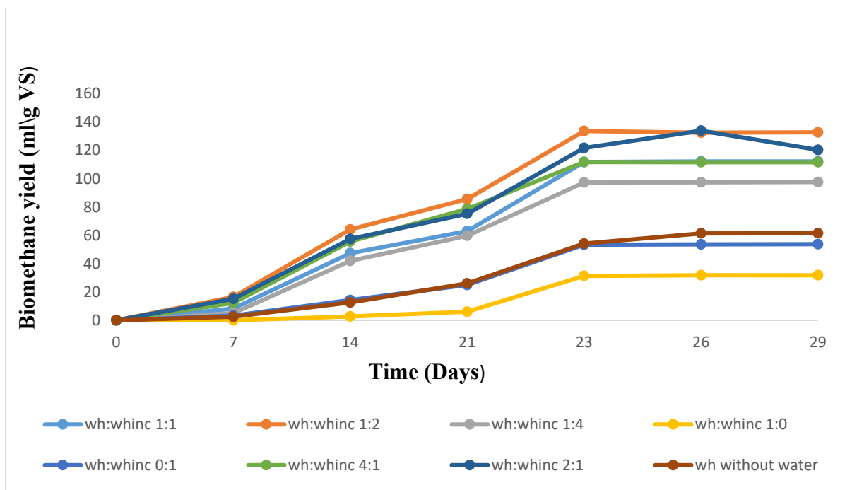
Fig. 7.1: Biomethane yield from anaerobic digestion of water hyacinth with water hyacinth inoculum.
