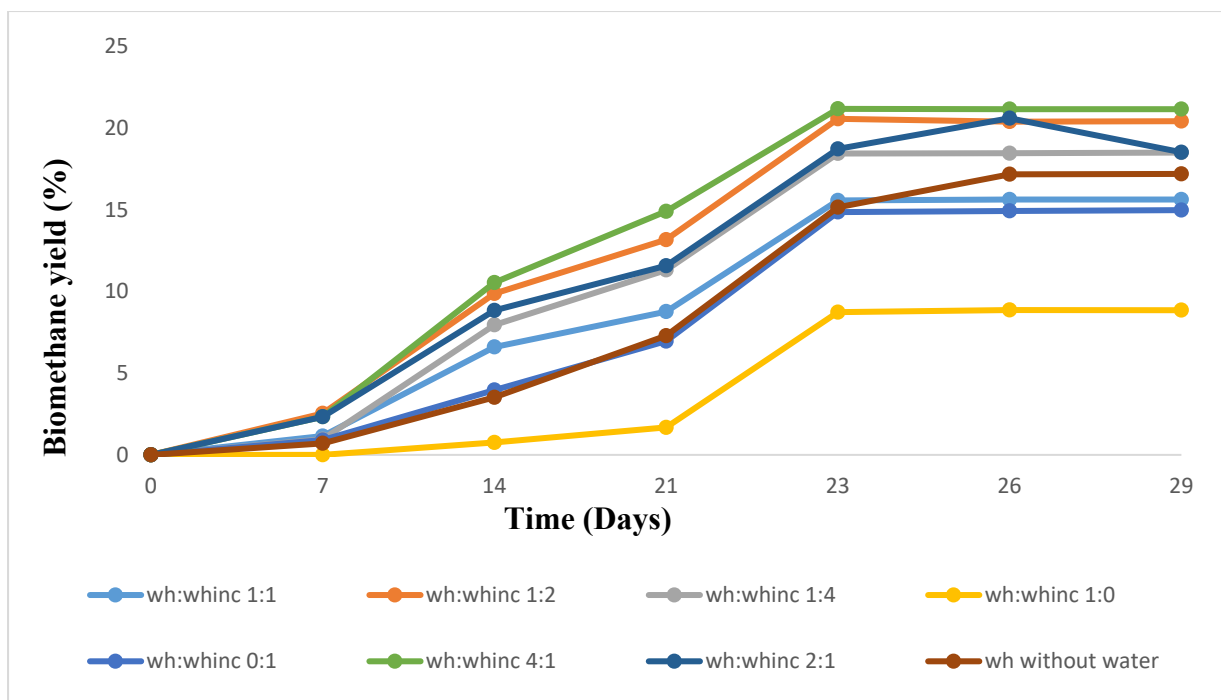
Fig. 7.2: Percentage biomethane yield in biogas from anaerobic digestion of water hyacinth with water hyacinth inoculum.
