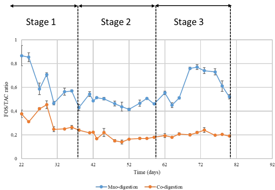
Fig. 6.4: FOS/TAC ratio for mono and co-digestion. Stage 1 – feeding once a week, stage 2 – feeding twice a week and stage 3 – feeding once a week with increased VS
