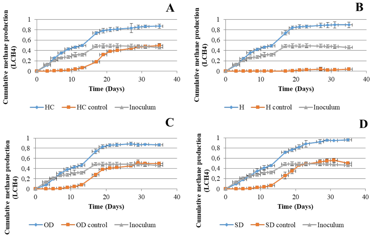
Fig. 4.2: Cumulative CH 4 production for physical pre-treatment methods; A – hand cut, B – homogenised, C –oven dried and D – sun dried, error bars represent standard deviation (n=3)
