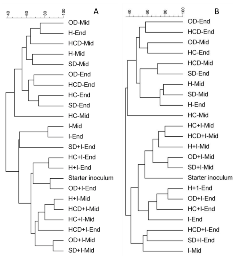
Fig. 5.3: Hierarchical cluster dendrogram (UPGMA) based on DGGE fingerprints of (A) archaeal 16S rRNA amplicons and (B) bacterial 16S rRNA amplicons representing archaeal and bacterial communities associated with various methods of substrate pre-treatment. OD, oven dried; H, homogenised; HCD, hand cut and decomposed; SD, sun dried; HC, hand cut; I, inoculum
