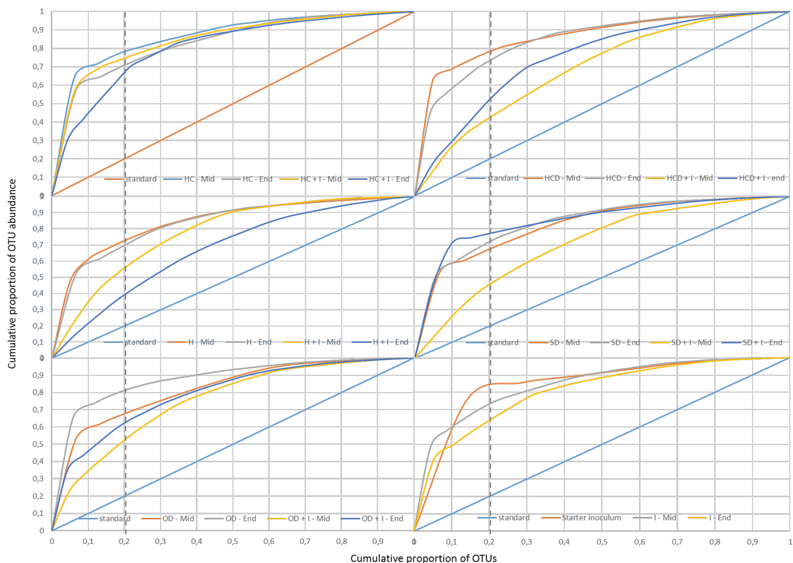
Fig. A5.2: Pareto-Lorenz distribution curves based on the bacterial DGGE profiles associated with various methods of substrate pre-treatment for graphical representation of the bacterial community evenness. Perfect evenness is illustrated as a straight line (standard). A dashed vertical line is plotted to evaluate the range of the Pareto value. OD, oven dried; H, homogenised; HCD, hand cut and decomposed; SD, sun dried; HC, hand cut; I, inoculum.
