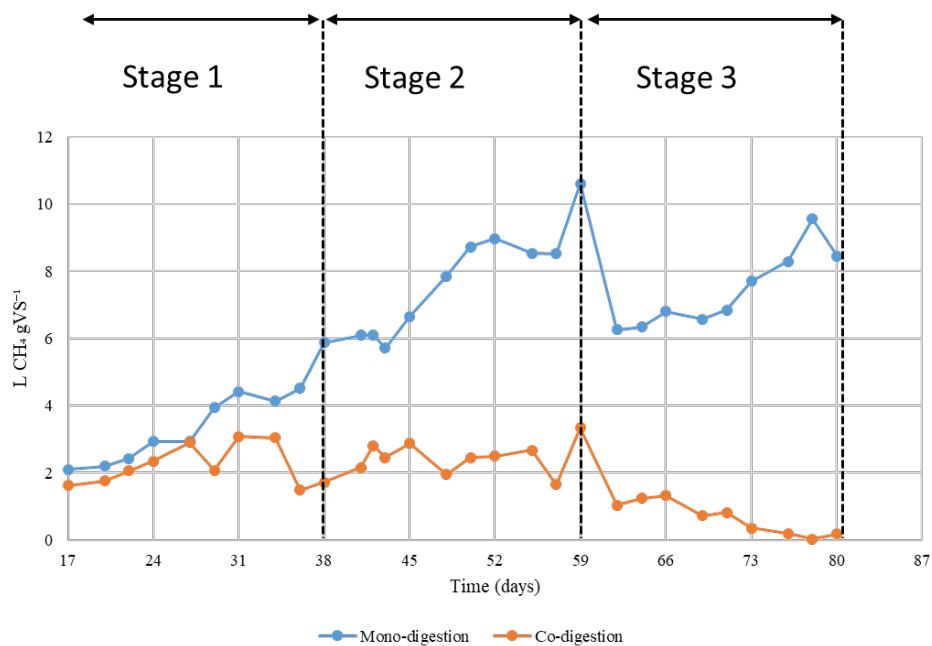
Fig. 6.3: LCH_4 gVS^{-1} for mono and co-digestion. Stage 1 – feeding once a week, stage 2 – feeding twice a week and stage 3 – feeding once a week with increased VS
