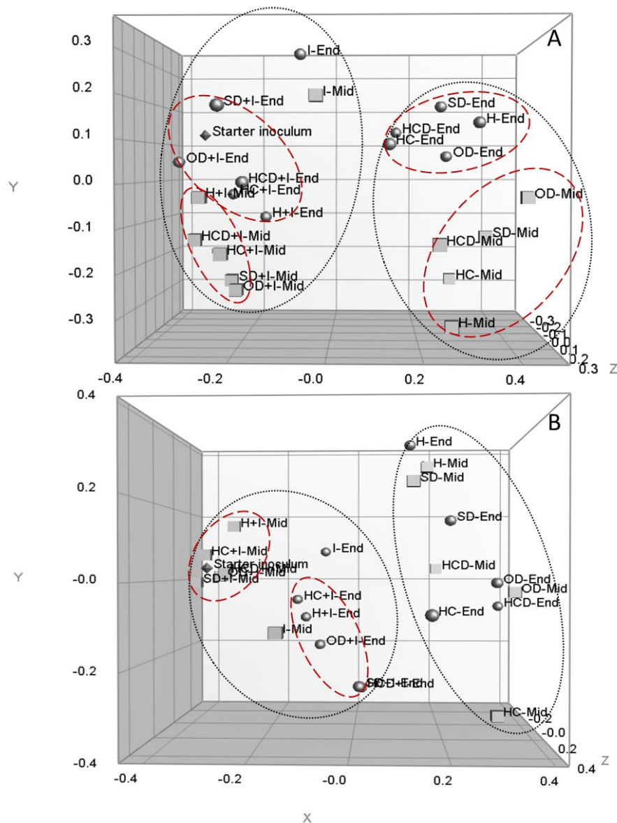
Fig. 5.4: Multi-dimensional scaling ordination plot based on the relative band positions on (A) archaeal and (B) bacterial DGGE profiles. Squares represent profiles obtained mid-way through the trial and circles represent profiles obtained at the end of the trial. OD, oven dried; H, homogenised; HCD, hand cut and decomposed; SD, sun dried; HC, hand cut; I, inoculum
