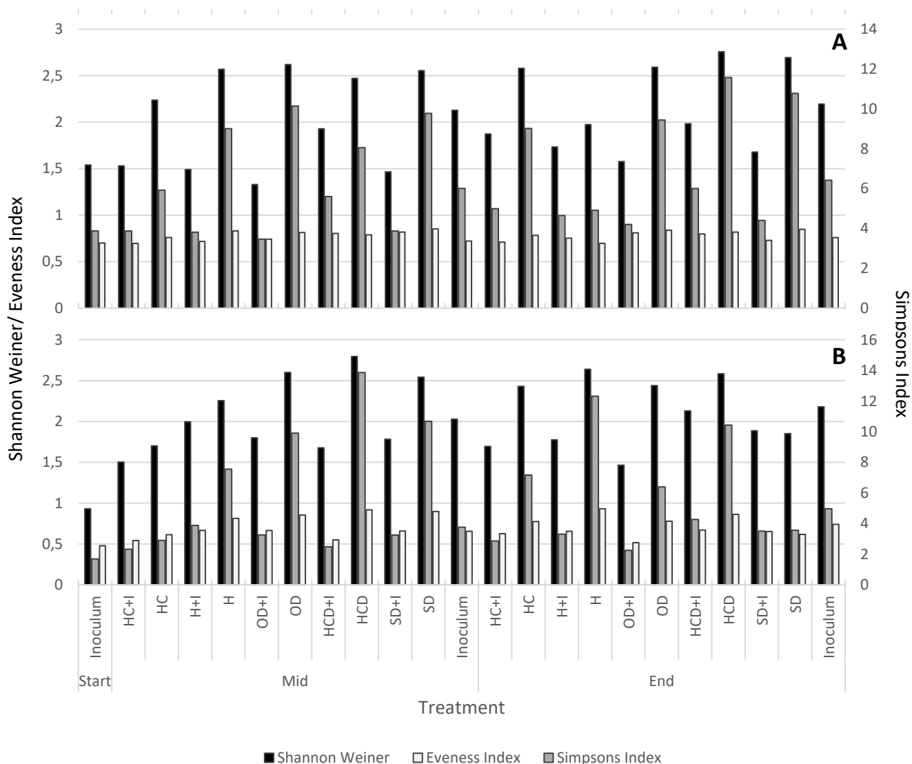
Fig. 5.5: (A) Archaeal and (B) bacterial diversity indices associated with various methods of substrate pre-treatment. OD, oven dried; H, homogenised; HCD, hand cut and decomposed; SD, sun dried; HC, hand cut; I, inoculum.
