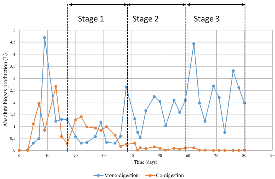
Fig. 6.2: Absolute biogas production from mono and co-digestion. Stage 1 – feeding once a week, stage 2 – feeding twice a week and stage 3 – feeding once a week with increased VS 4% TS.
