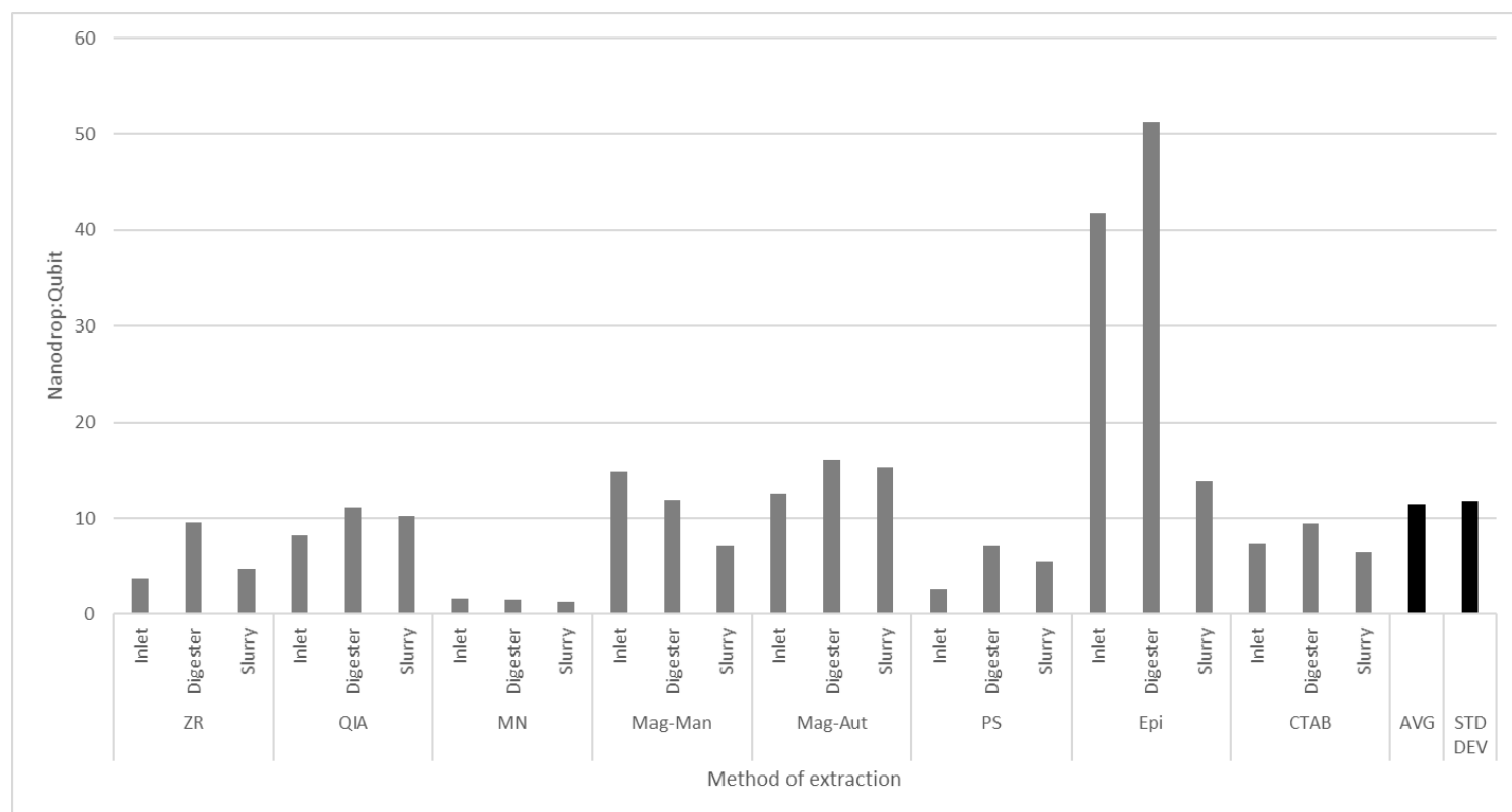
Fig. A2.1 Ratio of Nanodrop and Qubit measurements of DNA extracts from samples obtained from the inlet, digester and slurry using various methods of DNA extraction.
