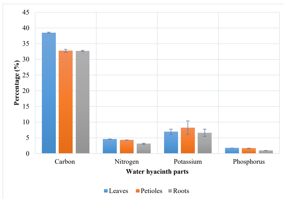
Fig. 3.1: Chemical analysis of different part of the plant, Error bars represent standard deviation (n=3)
