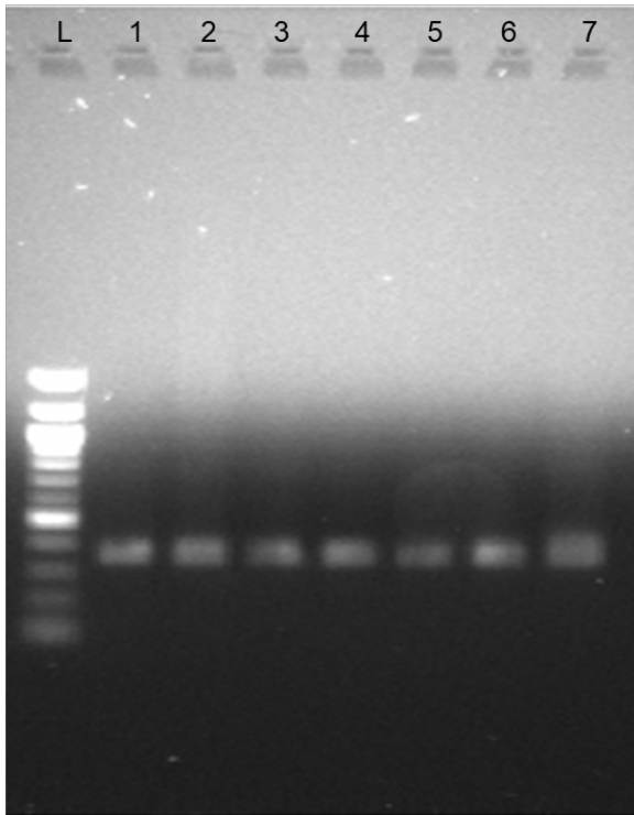
Fig. 8.4: PCR of the nifH gene fragment amplified from the digestate samples. L-100bp DNA ladder; 1, 2, 3, 4, 5, 6 & 7 – Different treatments of digestate samples
