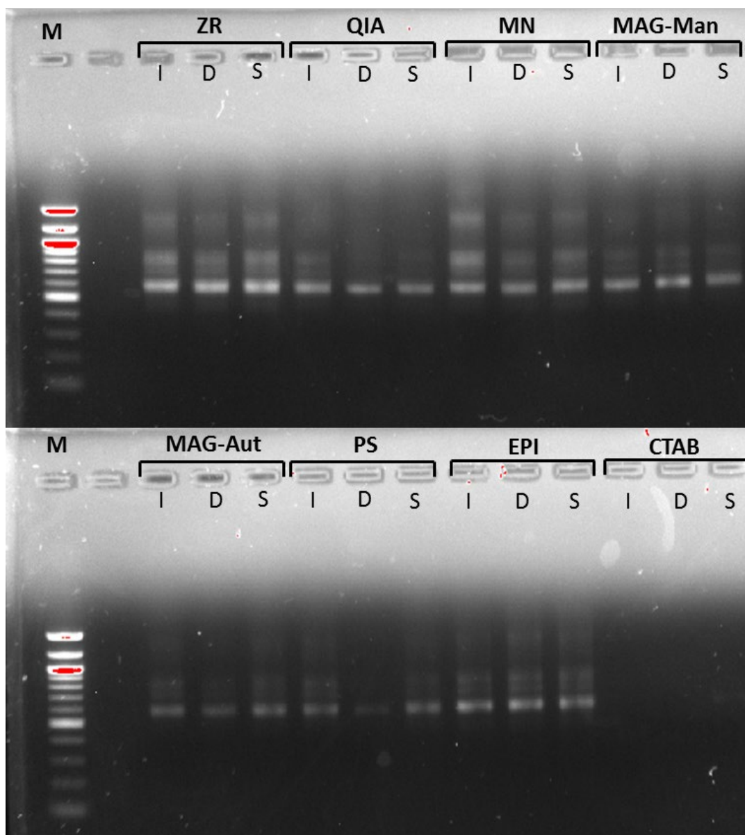
Fig. A2.2 PCR amplicons from samples obtained before, during and after anaerobic digestion using various DNA extraction methods (Primer pair: 341F-907R). M = DNA ladder; I = Inlet; D = Digester; S = Slurry; ZR = ZR Soil Microbe DNA MiniPrep – Zymo Research; QIA = QIAamp Fast DNA Stool Mini Kit – QIAGEN; MN = NucleoSpin Soil Kit – Macherey-Nagel; MAG-Man = MagMAX Total Nucleic Acid Isolation Kit – Manual – Thermo Fisher Scientific; MAG-Aut = MagMAX Total Nucleic Acid Isolation Kit – Automated – Thermo Fisher Scientific; PS = Powersoil DNA Isolation Kit – MO BIO Laboratories; EPI = Meta-G-Nome DNA Isolation Kit – Epicentre; CTAB = CTAB based extraction.
