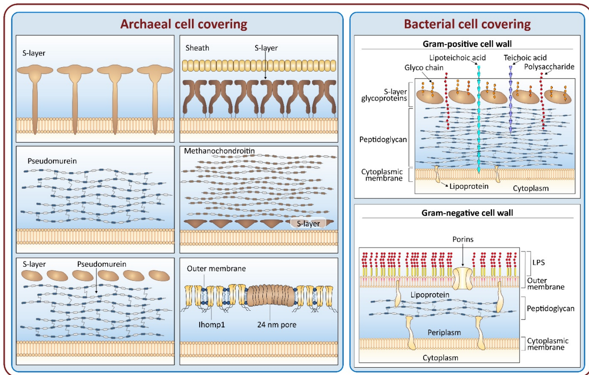
Fig. A2.3 Cell surface structure of archaeal and bacterial cells (adapted from Albers & Meyer, 2011).
