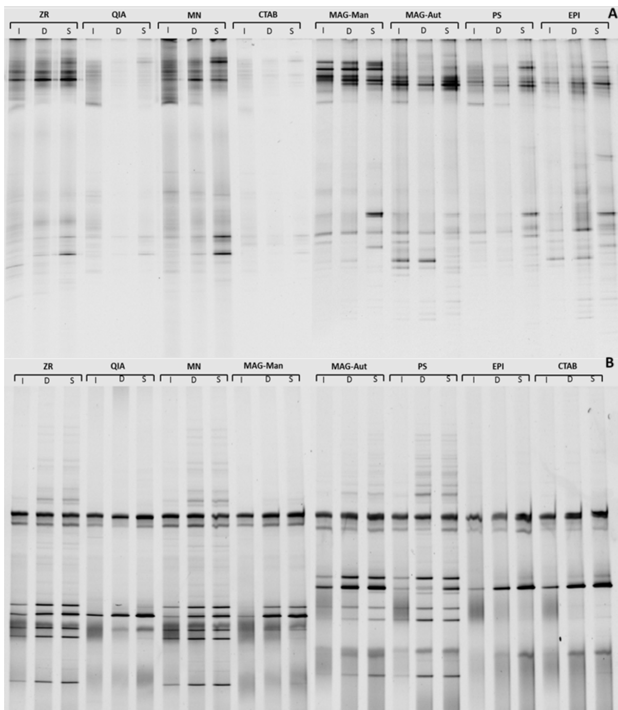
Fig. 2.3: DGGE banding patterns of (A) bacterial & (B) archaeal DNA isolated from samples obtained from the inlet, digester and slurry using various DNA extraction methods. I = Inlet; D = Digester; S = Slurry; ZR = ZR Soil Microbe DNA MiniPrep – Zymo Research; QIA = QIAamp Fast DNA Stool Mini Kit – QIAGEN; MN = NucleoSpin Soil Kit – Macherey-Nagel; Mag-Man = MagMAX Total Nucleic Acid Isolation Kit – Manual – Thermo Fisher Scientific; Mag-Aut = MagMAX Total Nucleic Acid Isolation Kit – Automated – Thermo Fisher Scientific; PS = Powersoil DNA Isolation Kit – MO BIO Laboratories; EPI = Meta-G-Nome DNA Isolation Kit – Epicentre; CTAB = CTAB based extraction.
