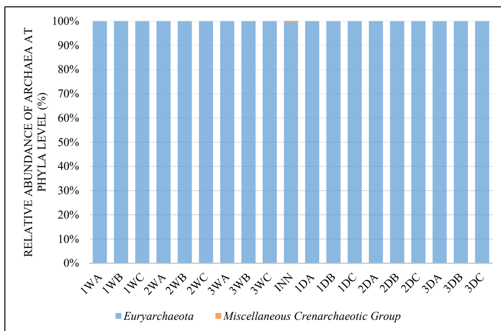
Fig.6.8: Relative abundance of archaea at phyla level for mono (W) and co digestion (D). A – Stage 1, B – stage 2 and C – stage 3, while 1 – beginning, 2 – mid and 3 – end of stage. INN – inoculum.
