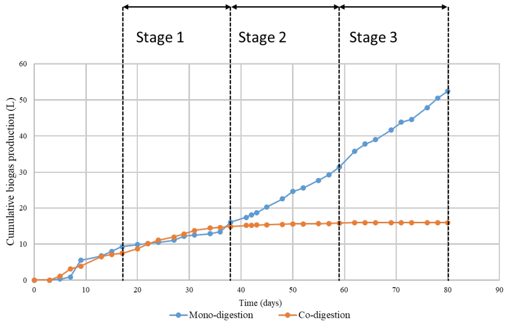
Fig. 6.1: Biogas production. Stage 1 – feeding once a week, stage 2 – feeding twice a week and stage 3 – feeding once a week with increased VS
