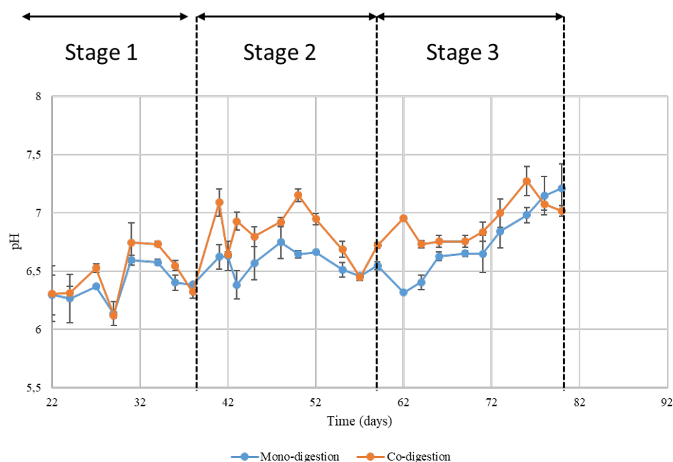
Fig. 6.5: pH of the two digesters. Stage 1 – feeding once a week, stage 2 – feeding twice a week and stage 3 – feeding once a week with increased VS
