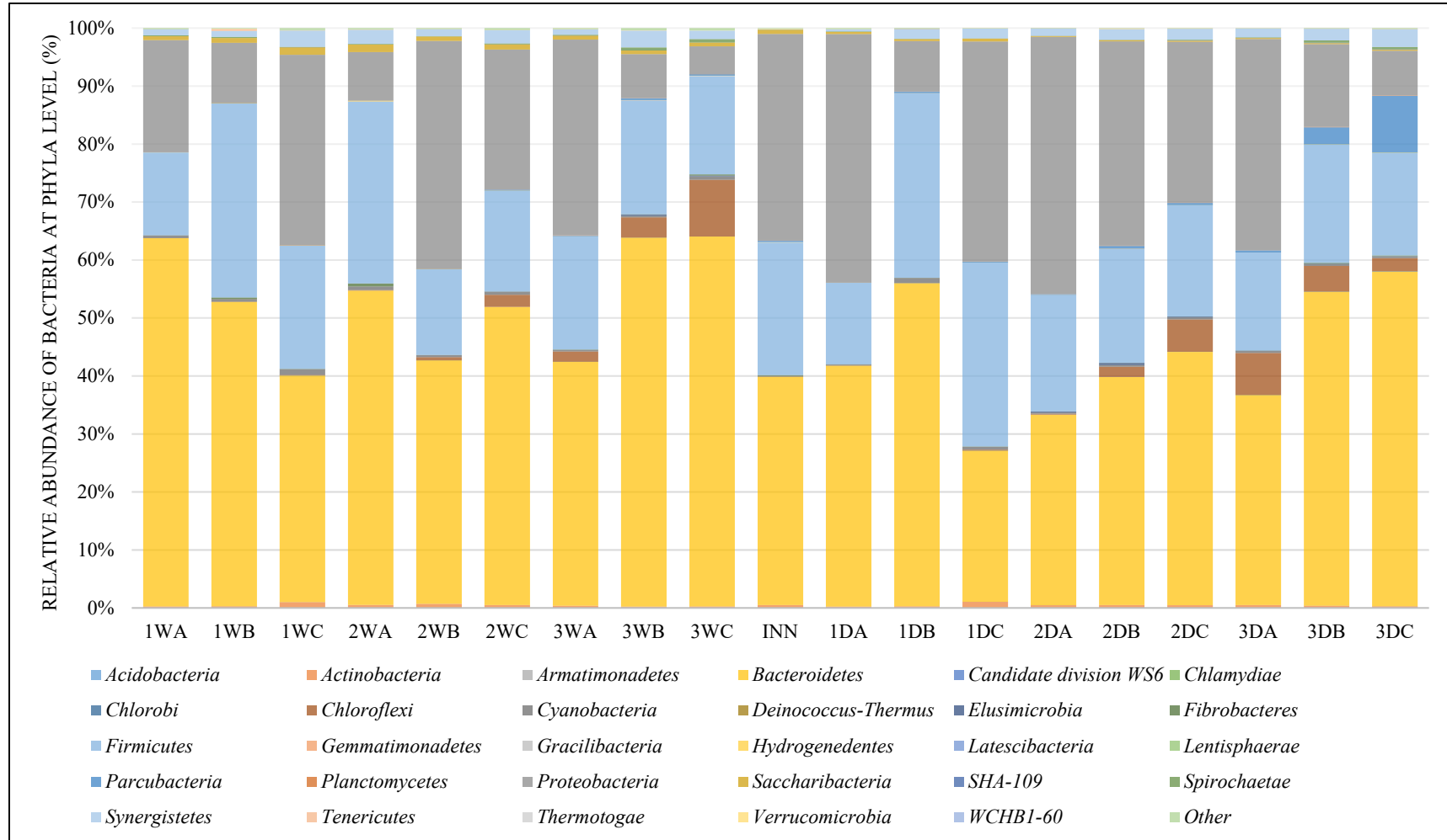
Fig. 6.6: Relative abundance of bacteria at phyla level for mono (W) and co digestion (D). A – Stage 1, B – stage 2 and C –stage 3, while 1 – beginning, 2 – mid and 3 – end of stage. INN – inoculum.
