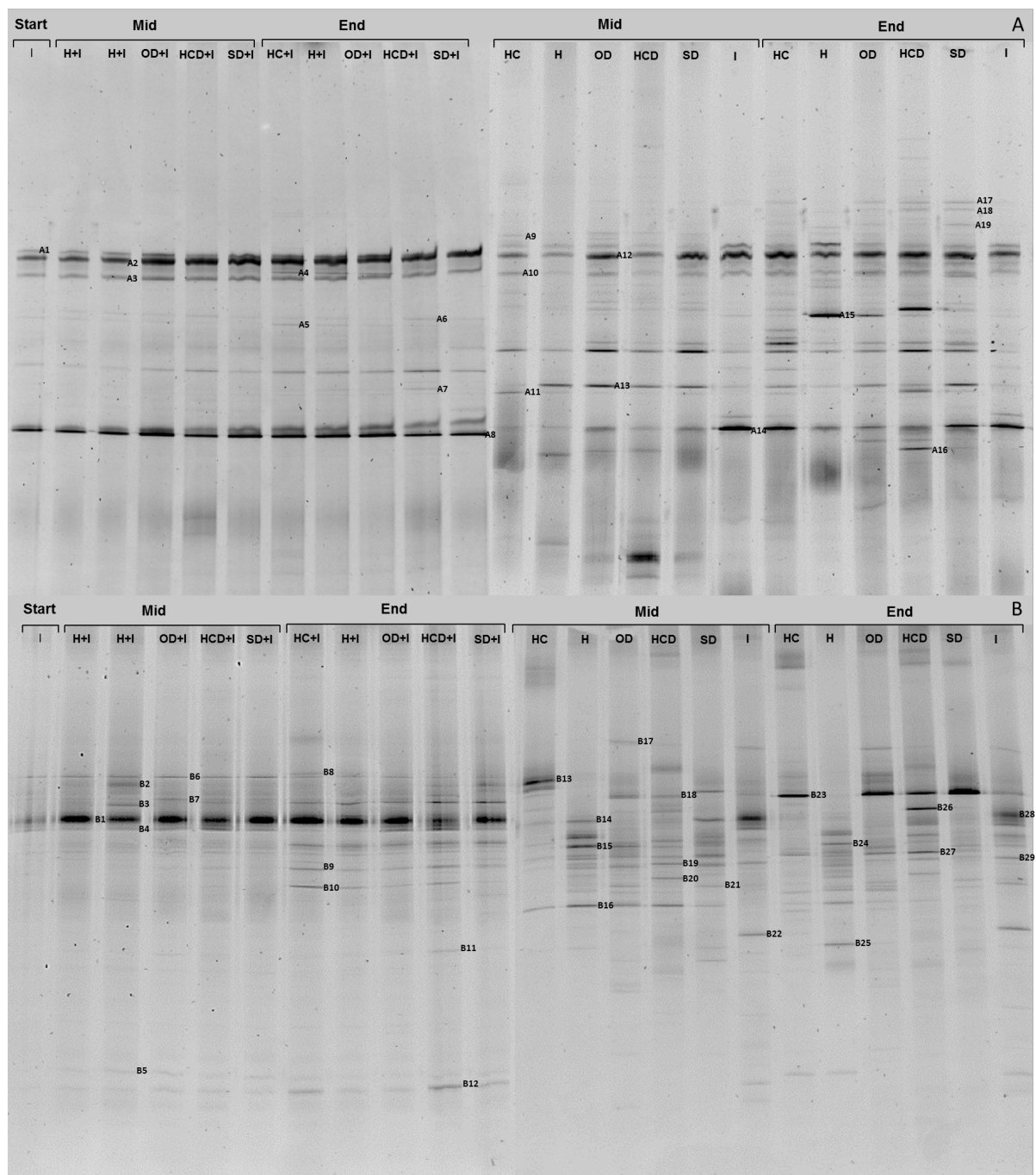
Fig. 5.2: PCR-DGGE image representing (A) archaeal and (B) bacterial communities associated with various methods of substrate pre-treatment. OD, oven dried; H, homogenised; HCD, hand cut and decomposed; SD, sun dried; HC, hand cut; I, inoculum.
