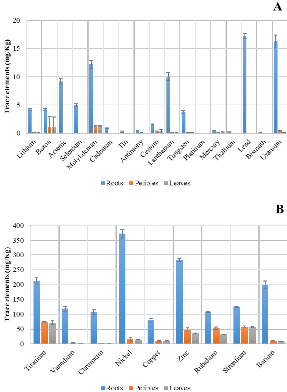
Fig. 3.2: Trace elements from different parts of the plant. A – Range of between 0.01-18 mg/Kg and B – Range of between 20-400 mg/Kg , Error bars represent standard deviation (n=3)
