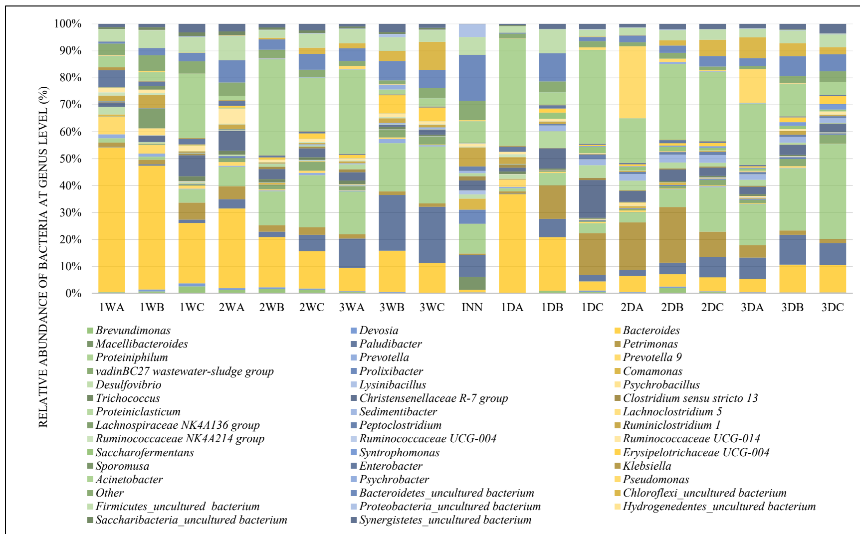
Fig. 6.7: Relative abundance of bacteria at genus level for mono (W) and co digestion (D). A – Stage 1, B – stage 2 and C – stage 3, while 1 – beginning, 2 – mid and 3 – end of stage. INN – inoculum.
