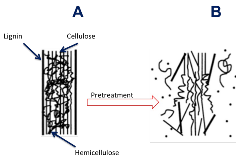
Fig. 4.1: Lignocellulosic structure with the three polymers. (A) and the effect of pre-treatment on lignocellulosic structure (B) (adapted from (Harmsen et al. , 2010)).
