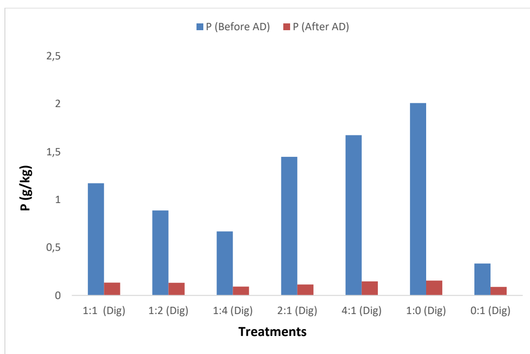
Fig. 8.2: Phosphorus content of the treatments before and after digestion
