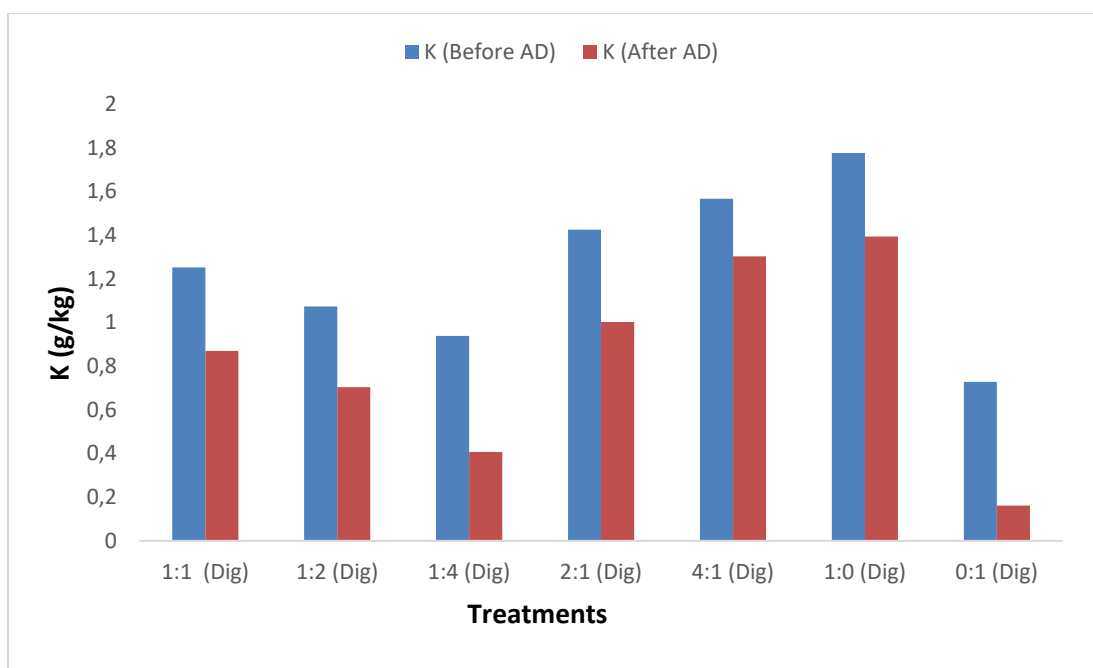
Fig. 8.3: Potassium content of the treatments before and after digestion
