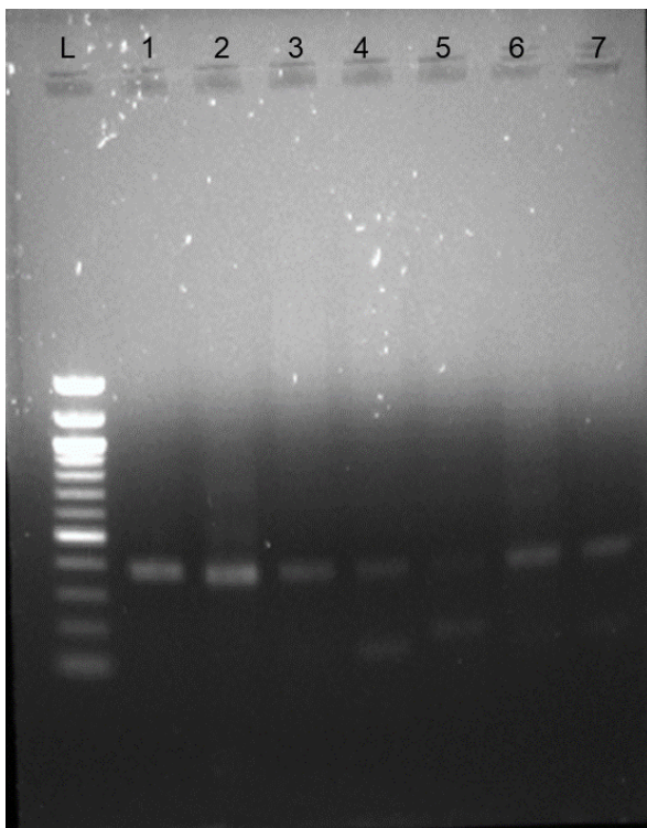
Fig. 8.5: PCR of the phoD gene fragment amplified from the digestate samples. L-100bp DNA ladder; 1, 2, 3, 4, 5, 6 & 7 – Different treatments of digestate samples
