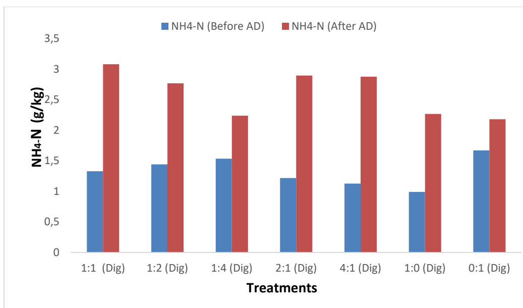
Fig. 8.1: Ammonium nitrogen content of the treatments before and after digestion
