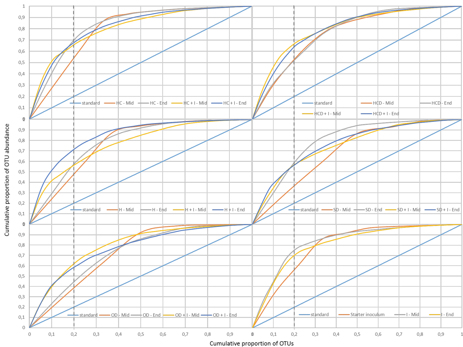
Fig. A5.1: Pareto-Lorenz distribution curves based on the archaeal DGGE profiles associated with various methods of substrate pre-treatment for graphical representation of the archaeal community evenness. Perfect evenness is illustrated as a straight line (standard). A dashed vertical line is plotted to evaluate the range of the Pareto value. OD, oven dried; H, homogenised; HCD, hand cut and decomposed; SD, sun dried; HC, hand cut; I, inoculum.
