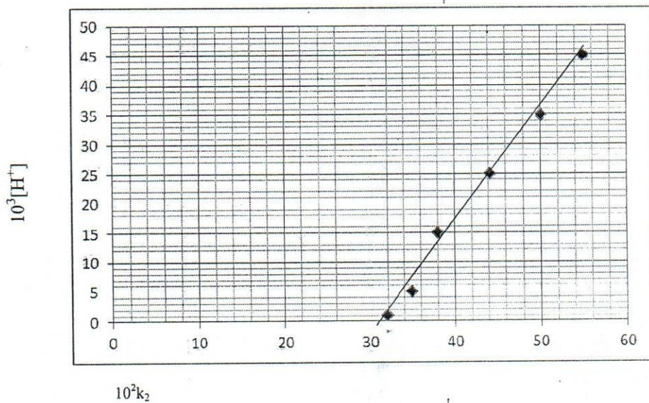
Figure 2 Graph of 10^2k_2 vs 10^3[H^+]
