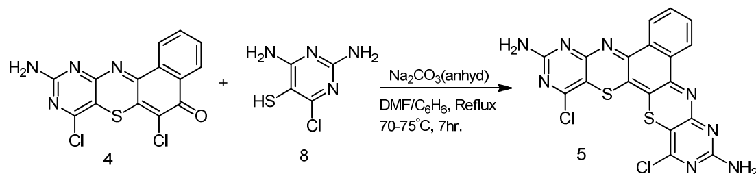
Figure 4b. The synthesis of 7,14-diamino-9, 12-dichloro-6, 8, 13, 15-tetraazabenz[a][1,4]benzothiazin-[3, 2, c] phenothiazine 5.
