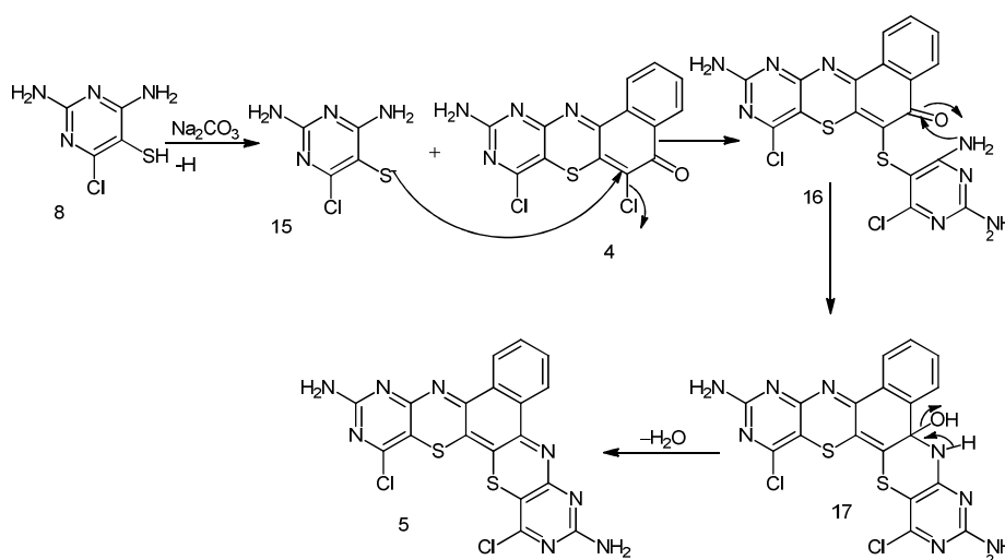
Figure 7. The reaction mechanism of 7, 14-diamino-9, 12-dichloro-6, 8, 13, 15-tetraazabenz[ a ] [1, 4] benzothiazin-[3, 2, c ] phenothiazine 5.
