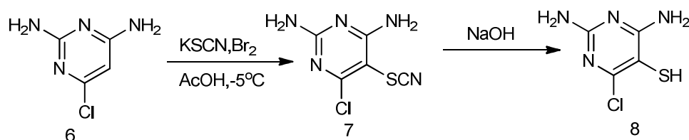
Figure 3. Synthesis of the key intermediate, 2, 6-diamino-4-chloro-pyrimidine-3-thiol 8.
